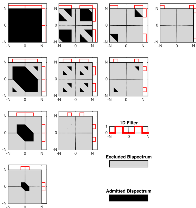
Figure 3. Effects of filtering on the bispectrum. Frequency axes are normalized relative to the Nyquist frequency ( N ), and the solid color depicts the part of the bispectrum respectively that is allowed to pass under a band-pass filter. (first to fourth rows) Greater filtering of high frequencies. (first to fourth column) Greater filtering of low frequencies. Note that both negative and positive frequencies contribute to the bispectrum.
