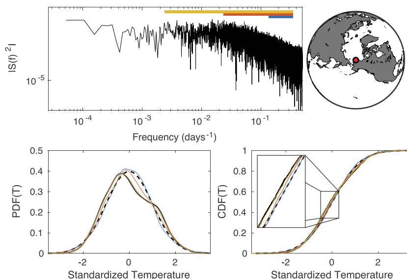
Figure 1. Filtering of radiosonde temperature time series and normality. (top) Power spectrum of a radiosonde time series of temperature at 850 mbar from Barrow, AK. The annual cycle is removed by notch filtering the annual frequency and its first two harmonics. The time series is then progressively filtered using a top-hat band-pass filter. The admitted frequency band for each filter is depicted by color bars indicating frequencies of 1/3 – 1/7 days ^{-1} (blue), 1/3 – 1/40 days ^{-1} (orange), and 1/3 – 1/400 days ^{-1} (yellow). (bottom) The probability density function and cumulative density function are depicted for winter (DJF) temperatures for the full data (solid black line), the filtered time series (solid colored lines), and a standardized normal distribution (dashed line).
