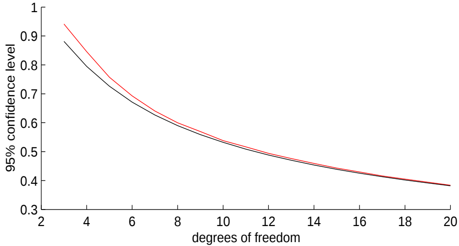
Figure 4-9: The 95% confidence level for linear coherence (black) and nonlinear coherence (red) as a function of the degrees of freedom (DOF). For large DOF the difference between the difference between linear and nonlinear coherence becomes negligible.
