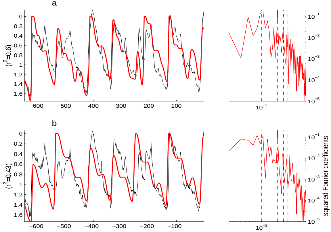
Figure 5-5: Model results (red, thick line) where parameters are chosen to maximize the cross-correlation with EOF1 (black, thin line) a Model results using an orbital forcing comprised of obliquity and precessional variations ( \mathcal{F}_{op} ) along with the periodogram of the model results. b Results when the model is only forced by obliquity ( \mathcal{F}_o ). The vertical dashed lines at right indicate frequencies of 1/100, 1/70, 1/41, 1/27, and 1/23KY. Concentrations of variability exist at bands near each of the indicated frequencies for both model results a and b.
