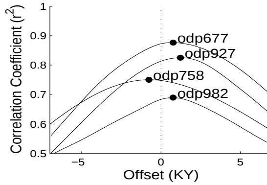
Figure 3-5: Lagged cross-correlation between sets of benthic and planktic \delta^{18}\text{O} records measured in the same core. Positive values indicate a benthic lead.
