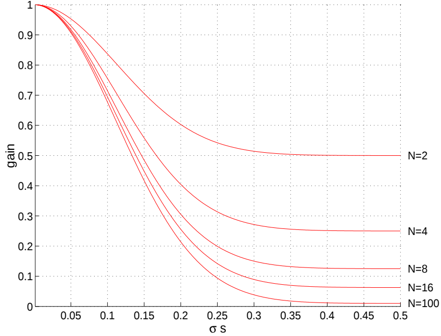
Figure 3-18: The expected gain, Eq 3.39, plotted against frequency, s , times the standard deviation of the relative age-model jitter, \sigma . Plots are for averaging N = 2, 4, 8 , and 16 records. The gain scales equivalently with both \sigma and s ( \sigma s \sim \sqrt{-\ln g} ) so that it is more general to plot the gain against \sigma s . For small \sigma s the gain approaches one, while for large \sigma s the gain asymptotes to 1/N — the expected behavior for perfect synchronization and complete phase randomization respectively.
