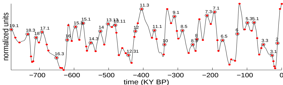
Figure 3-19: The SPECMAP \delta^{18}\text{O} stack [Imbrie et al., 1984] with each of its ACPs labeled as red dots. The thirty ACPs used to construct the high-resolution EOF1 are indicated by black circles and are numbered according the decimal notation used for the SPECMAP stack. Time goes from left to right and the units are normalized.
