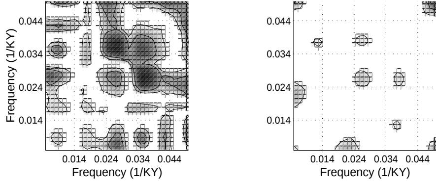
Figure 3-15: The auto-bicoherence of \psi(t) before (left) and after (right) orbital-tuning. Significant auto-bicoherence is indicated by light-shading for the off-diagonal and dark-shading for the on-diagonal.
