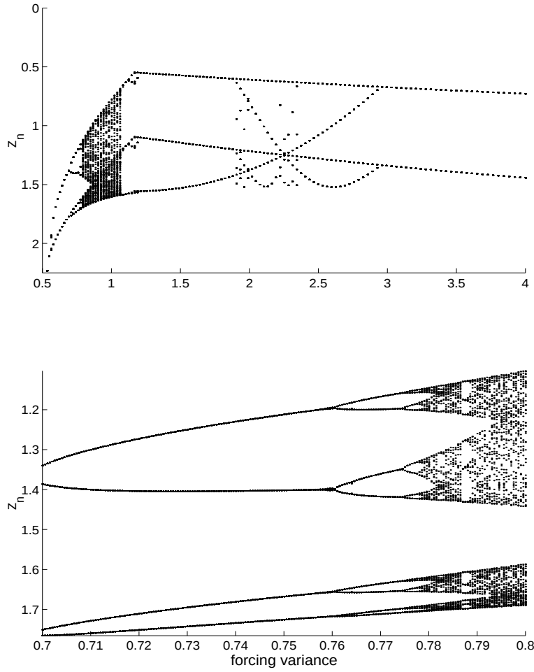
Figure 5-17: An orbit diagram for the model where the variance of each local maximum in ice-volume is plotted against forcing variance. The forcing is a 40KY sine wave, and a local maximum in ice-volume occurs exactly once for each forcing cycle. Thus the number of distinct dots in a vertical row indicates the period of the model response. top As the forcing variance increases from 0.5 a period doubling route to chaos is observed, but at values above 1.1, the model response again becomes periodic. For forcings above 3, the response simplifies and is periodic at 80KY. bottom Zooming in on the interval between 1.2 and 1.4 shows the period doubling route to chaos more clearly.
