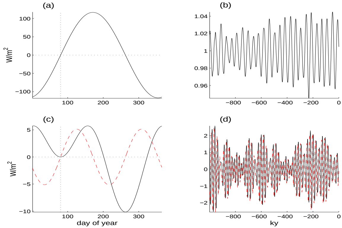
Figure 2-17: Similar to Figure 2-16 but for P_1 — the inter-hemispheric gradient in insolation. a, b: the leading set of singular vectors, termed the obliquity vectors, account for 99.4% of the variance in the insolation gradient. a, The leading seasonal obliquity vector is a sine wave with an annual period, amplitude of 110 \text{ W/m}^2 , and zero phase at the vernal equinox (vertical dotted line) — during the equinoxes there is no inter-hemispheric gradient in insolation. The seasonal obliquity vector is zero mean because changes in obliquity redistributes insolation between the hemispheres, but does not change global insolation values. b, the annual variability in insolation gradient is modulated by up to \pm 4\% due to changes in obliquity. Because obliquity is always positive, the associated secular singular vector is also a positive function. c,d: The precessional vectors together explain 0.5% of the inter-hemispheric gradient. c The seasonal variability is mostly controlled by changes in the timing of the inter-hemispheric insolation gradient. As the vernal equinox is fixed to March 20th and, by definition, has no inter-hemispheric gradient in insolation its value must be zero. The doubly-periodic nature of the seasonal vectors and the large excursion near the autumnal equinox is explained in the text. d Changes in climatic precession can add or subtract up to 20 \text{ W/m}^2 from the inter-hemispheric insolation gradient. Note the precession singular vectors are zero mean because precession variations do not affect annual mean insolation at any latitude.
