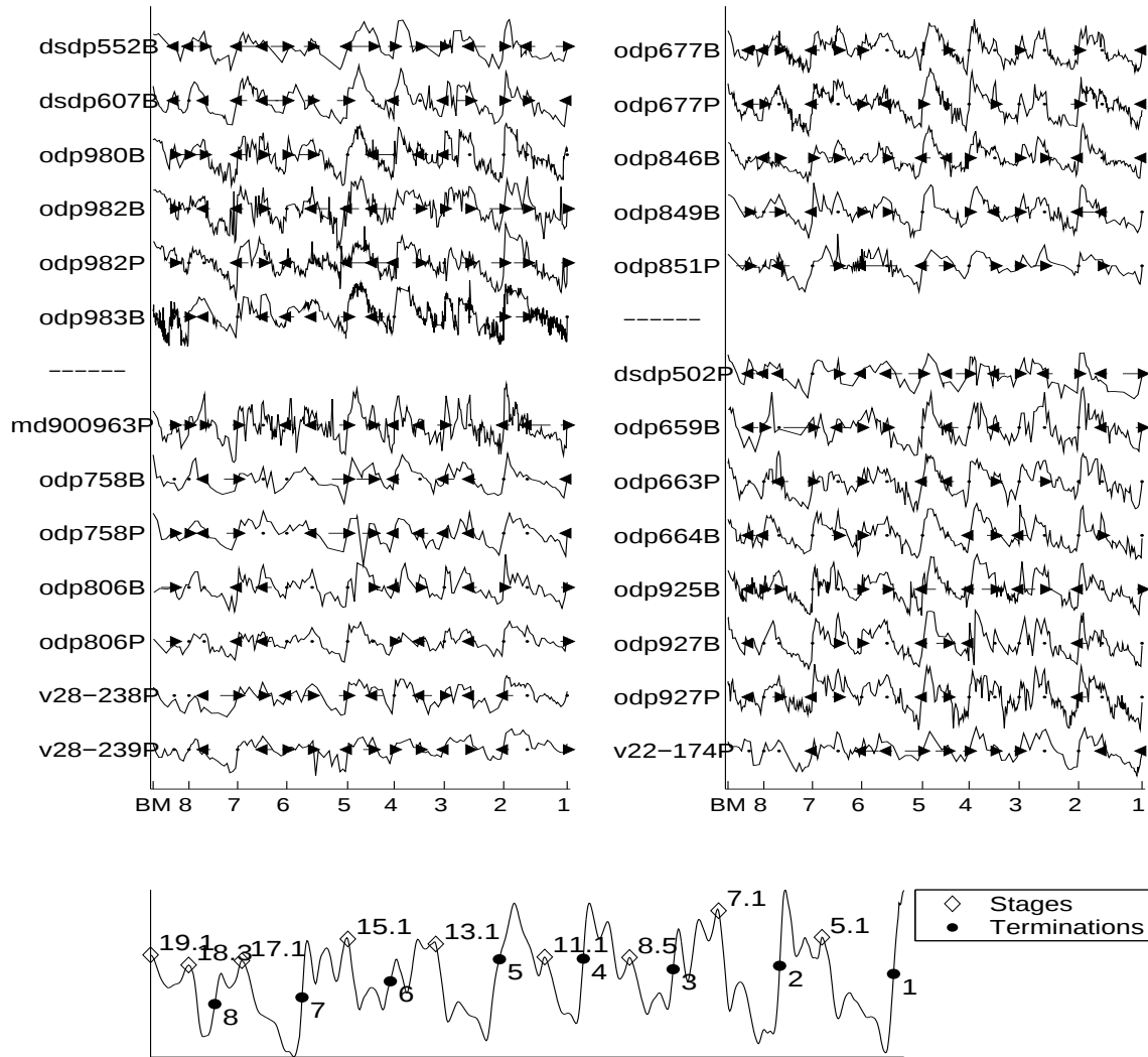
Figure 3-2: The \delta^{18}\text{O} isotope records, grouped into the four geographic categories shown in Figure 3-1: the North Atlantic (top left), Eastern Equatorial Pacific (top right), Indian and Western Equatorial Pacific (bottom left), and Equatorial Atlantic Oceans (bottom right). As described in the text, simultaneity between all records is enforced at 17 isotopic events. The ordinate is labeled with the B-M boundary location and termination numbers. The abscissa is to scale, and the \delta^{18}\text{O} records are vertically off-set from one another. The arrows at each event indicate how the age-model was adjusted from a linear age-depth relationship beginning with stage 18.3 and working toward stage 5.1. The letters B and P are appended to the record name to indicate it as benthic or planktic. Bottom panel is the SPECMAP \delta^{18}\text{O} stack oriented such that upward indicates lighter \delta^{18}\text{O} (inter-glacial). The SPECMAP stack is labeled with each of the 17 events for which ages are later estimated and the ordinate is arbitrary. Note that in this paper, time always increases to the right.
