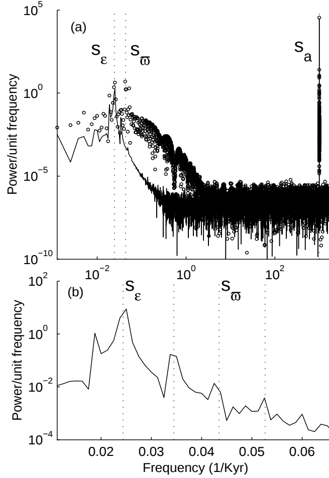
Figure 2-9: Periodograms of mean diurnal insolation plus a small amount of white noise. (a), Solid line is from insolation at 65^\circ\text{N} , while circles are from insolation passed through a \nu th-law device with \tau = 250 \text{ Watts/m}^2 and \nu = 1 . After rectification, low frequency energy at the obliquity band ( s_\epsilon ) is enhanced, and energy at the precession band ( s_\omega ) now appears. The ordinate and abscissa are logarithmic. For plotting purposes, an exponentially diminishing number of periodogram estimates are shown for frequencies above 1/10 \text{ kyr} except near the annual cycle and its first harmonic where full resolution is used—no significant structural changes result. (b), Periodogram of insolation at 85^\circ\text{N} . Vertical lines from left to right are centered on the obliquity bands at 1/41 and a minor side-band at 1/29 \text{ kyr} [Melice et al. , 2001] and precession at 1/23 and 1/19 \text{ kyr} . The abscissa is linear, and for visual clarity, only the low-frequencies are shown. The seasonal cycle, s_a , is so much more powerful than any other insolation frequency (other than the diurnal) that its rectification is of greatest concern, but all frequencies are susceptible to such effects.
